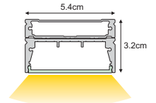
PRH.020 ANTISLIPPER for vertical installation (as extra)
